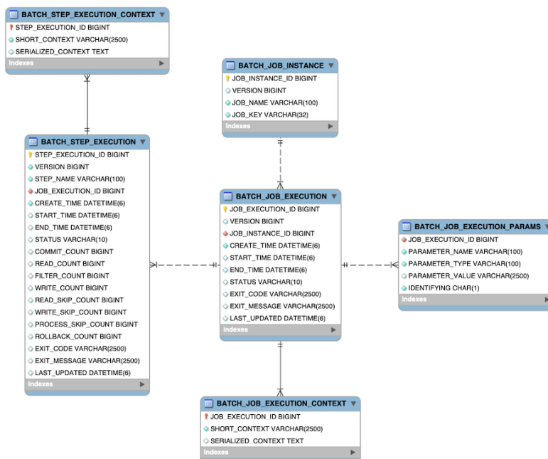
Figure 35. Spring Batch Meta-Data ERD
